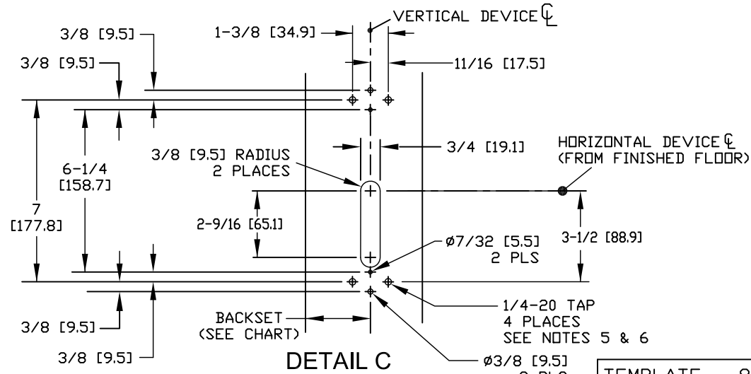
DETAIL B DOOR TOP DEVICE SIDE MACHINING & INTERNAL MECHANISM CLEARANCE
