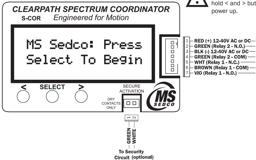
FIGURE 1 Wiring Diagram
